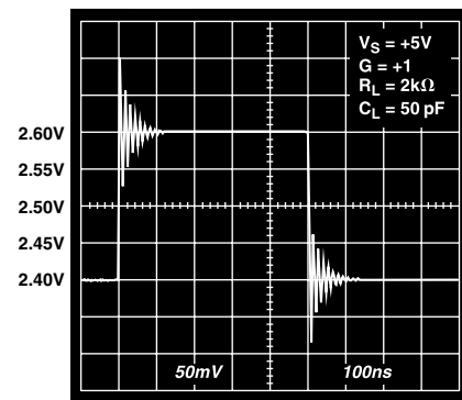
Figure 3. 200 mV Step Response: C_L = 50 \text{ pF}
