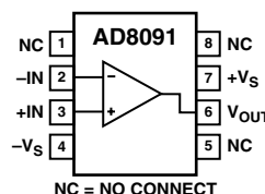
\mu SOIC-8 and SOIC-8 (RM-8, R-8)
