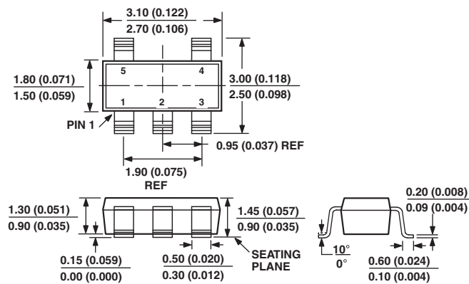
5-Lead Plastic Surface Mount (RT-5)
