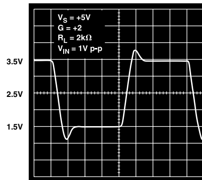
TPC 22. Large Signal Step Response; V_S = +5\text{ V} , G = +2
