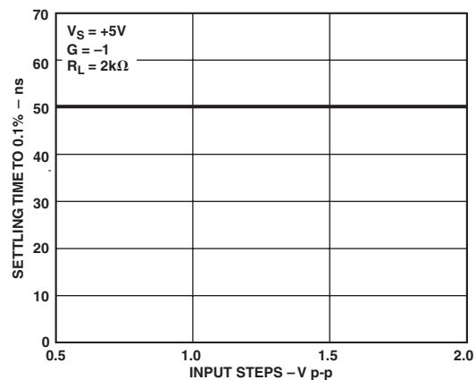
TPC 17. Settling Time vs. Input Step
