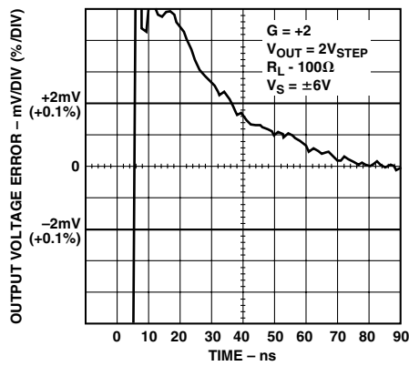
Figure 34. Settling Time; V_S = \pm 6.0 V
