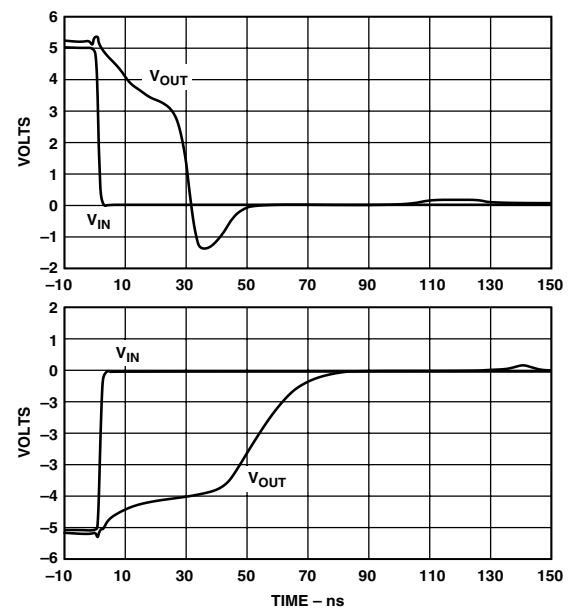
Figure 37. Overload Recovery; V_S = \pm 6 V , G = +2 , R_L = 100 \Omega , V_{IN} = 5 V_{p-p} , T = 1 \mu s
