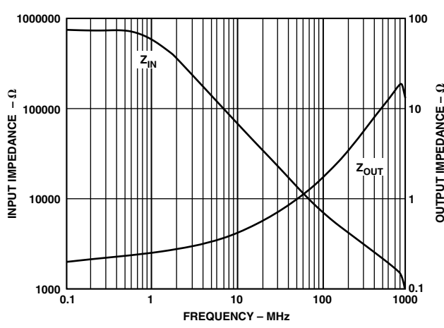
Figure 36. Input and Output Impedance vs. Frequency
