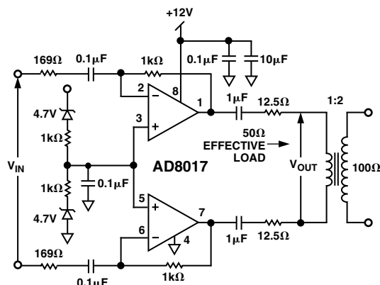
Figure 39. Single +12 V Supply ADSL Remote Terminal Transmitter
