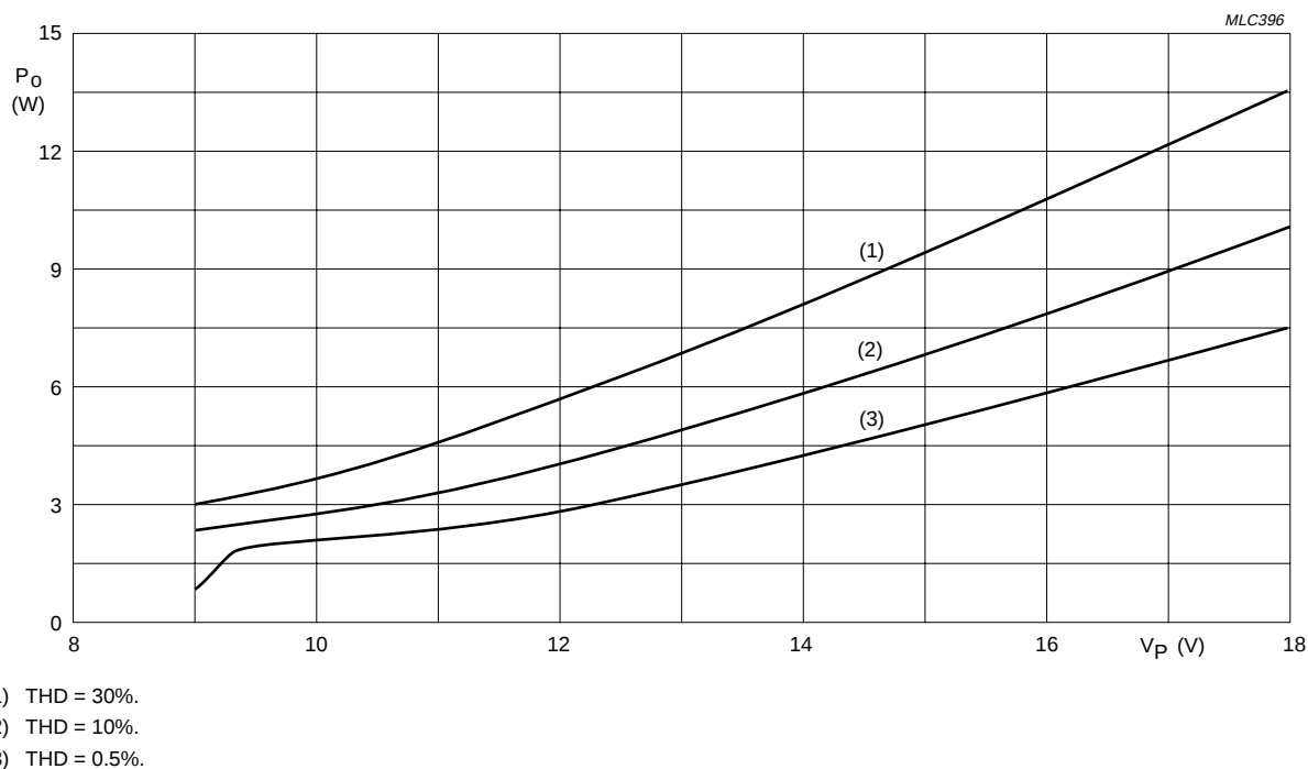
Fig.9 Output power as a function of supply voltage; R_L = 4\ \Omega .
