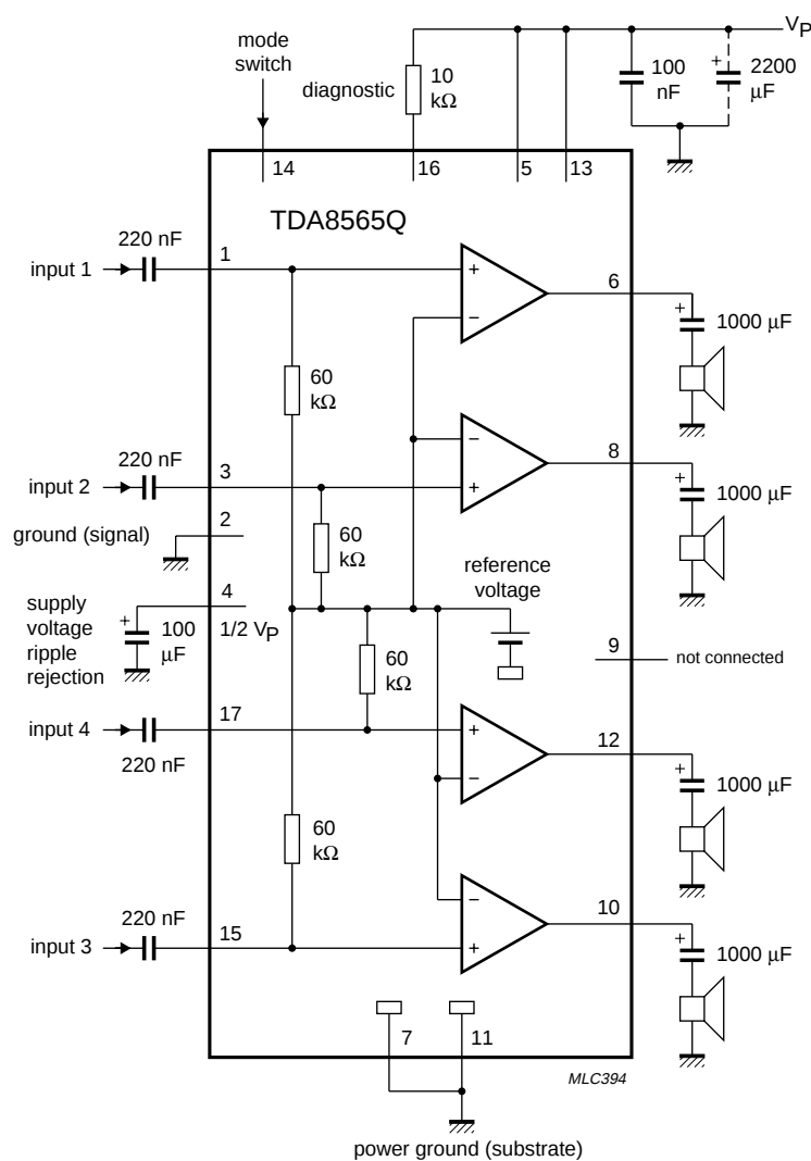
Fig.14 Application circuit diagram.
