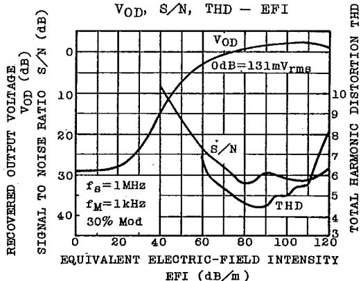
V_{OD}, S/N, THD - EFI
