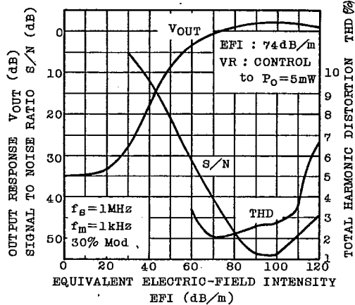
V_{OUT}, S/N, THD - EFI
