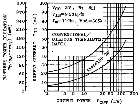
P_D(BATTERY), I_{CC} - P_{OUT} CHARACTERISTIC COMPARISON
