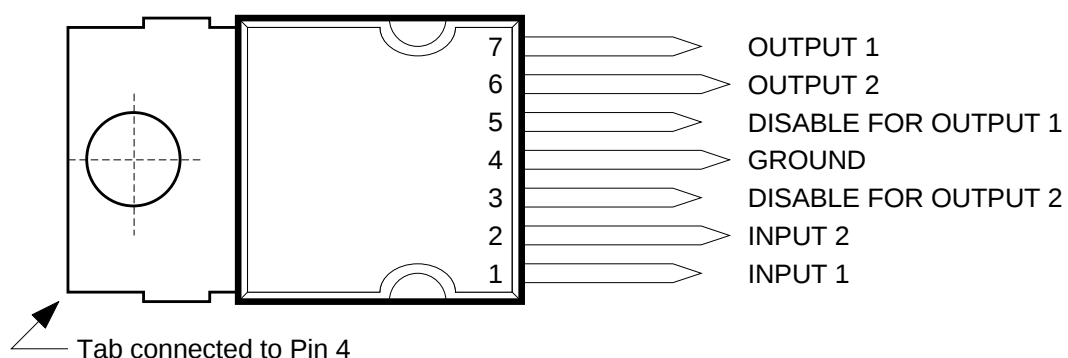
Figure 1. Pin Connections
