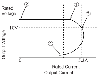
Fig2. Output Voltage/Current
