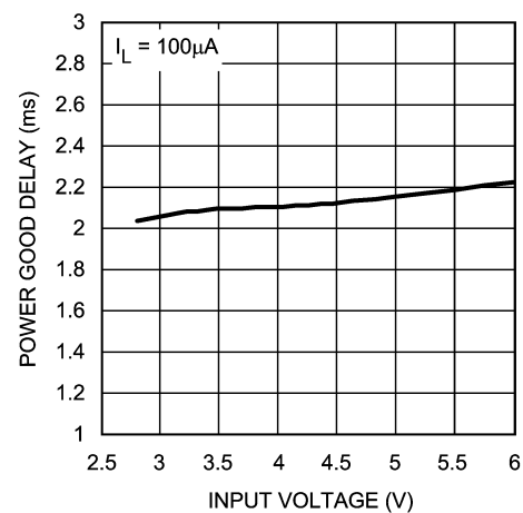
Power Good Delay vs. Input Voltage
