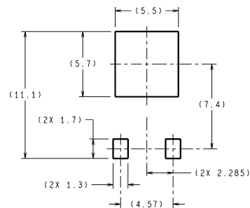
6-Pin LLP NS Package Number LDE06A
