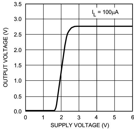
Dropout Characteristics
