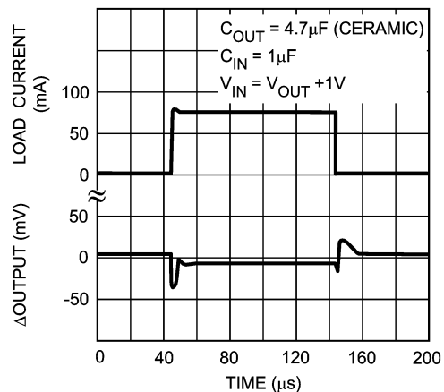
Load Transient
