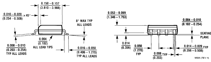
8-Pin Small Outline Package Order Number LMC6082AIM or LMC6082IM NS Package Number M08A
