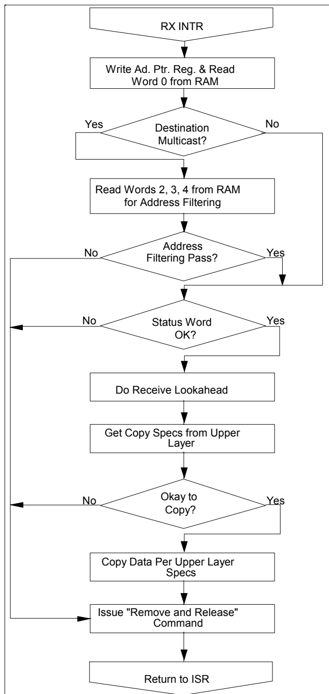
Figure 10.2 - RX INTR
