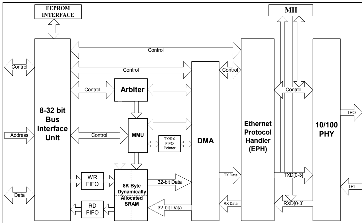
Figure 3.2 - Block Diagram
