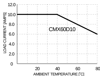
Max. Load Current vs. Temp.
