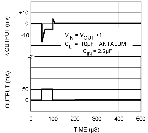
Load Transient
