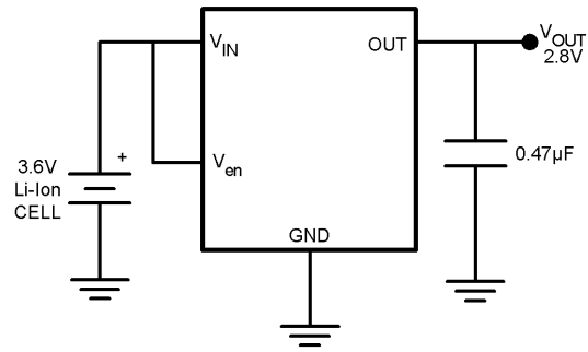
FIGURE 2. Single-Cell Regulator
