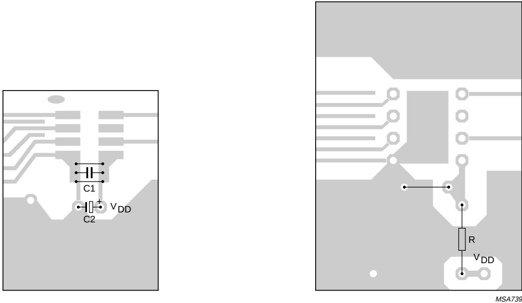
Fig.7 Recommended printed-circuit board layouts.
