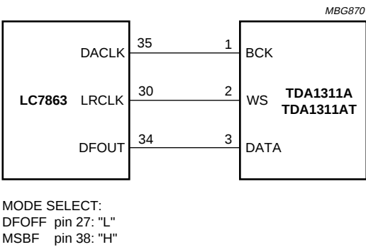
Fig.14 Sanyo LC7863 decoder (1FS).
