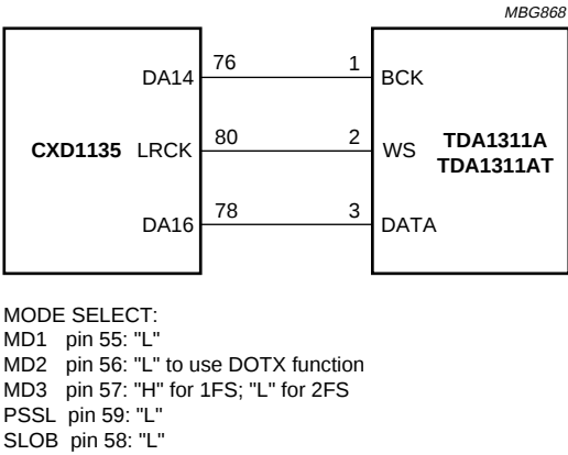
Fig.12 Sony CXD1135 decoder (1FS) and digital filter (2FS).
