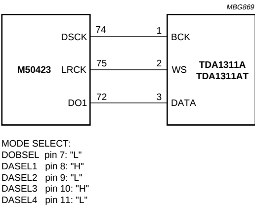
Fig.13 Mitsubishi M50423 decoder (1FS) and digital filter (4FS).
