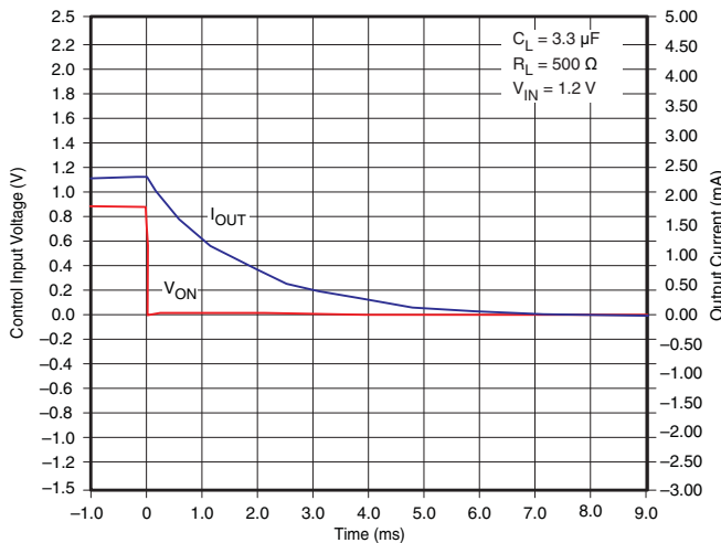
Figure 32. t_{OFF} Response
