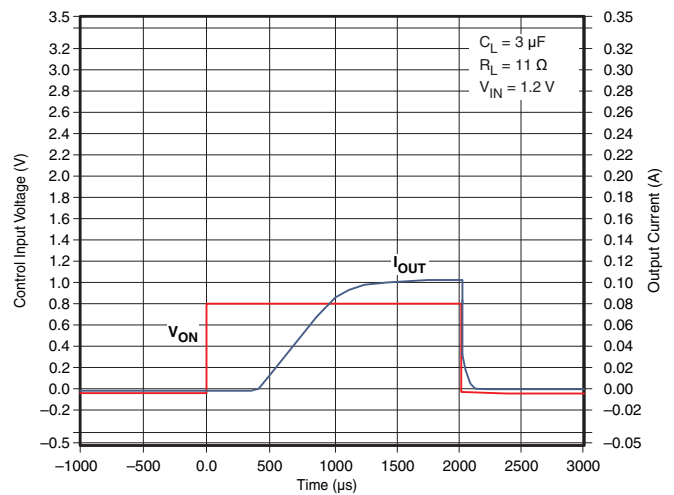
Figure 49. t_{ON} Response
