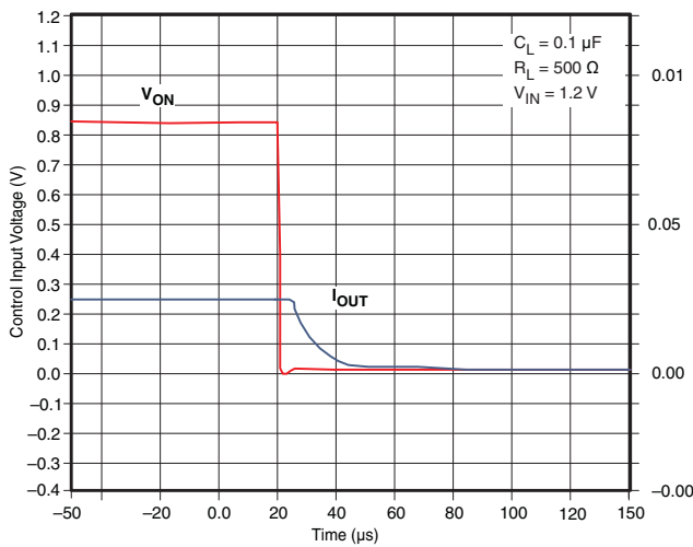
Figure 54. t_{OFF} Response
