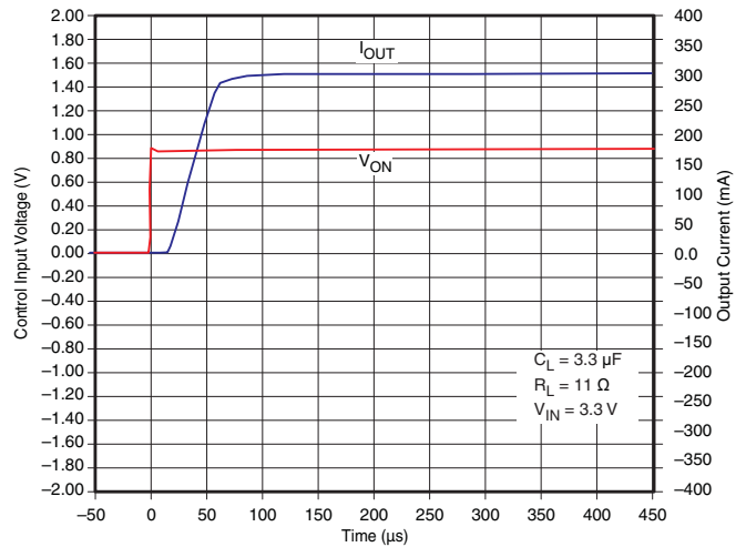
Figure 21. t_{ON} Response
