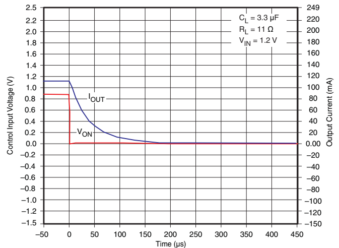
Figure 33. t_{OFF} Response
