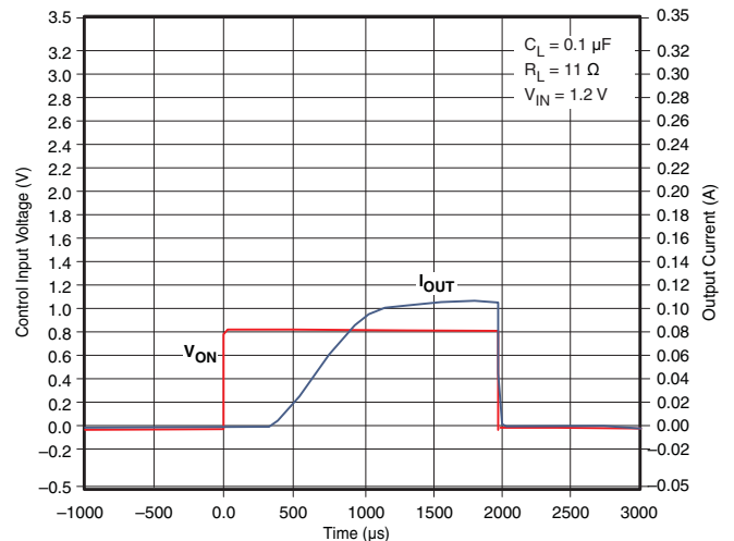
Figure 47. t_{ON} Response
