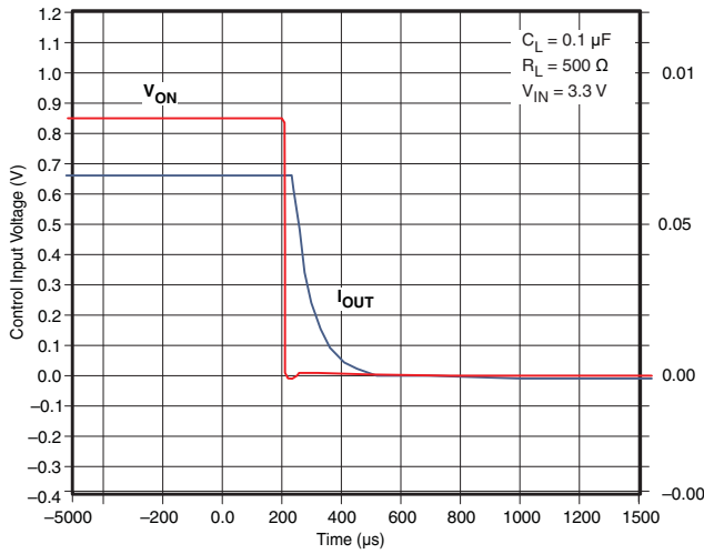
Figure 50. t_{OFF} Response
