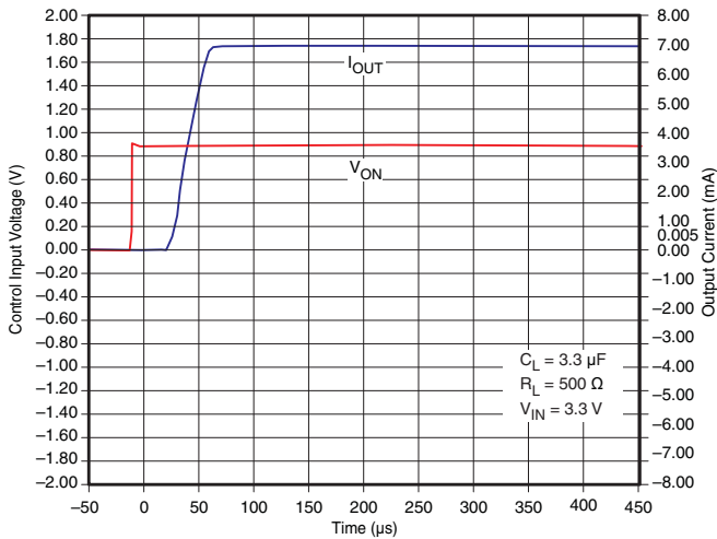
Figure 20. t_{ON} Response
