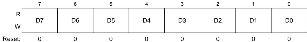
Figure 4-8. Linear Byte Post Increment Register (LBP)
