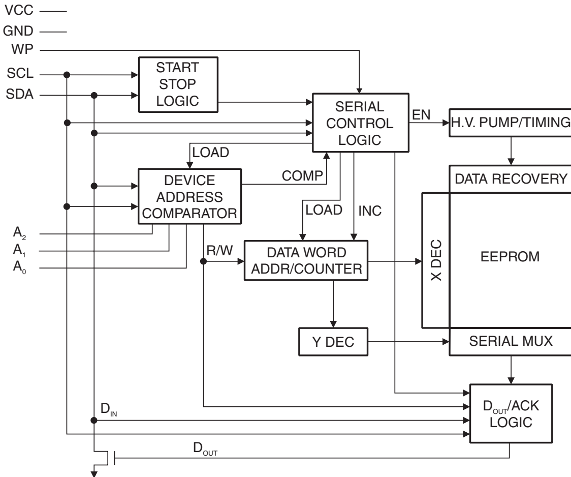
Figure 0-1. Block Diagram
