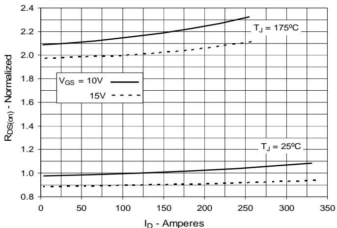
Fig. 5. R_{DS(on)} Normalized to I_D = 125A Value vs. Drain Current
