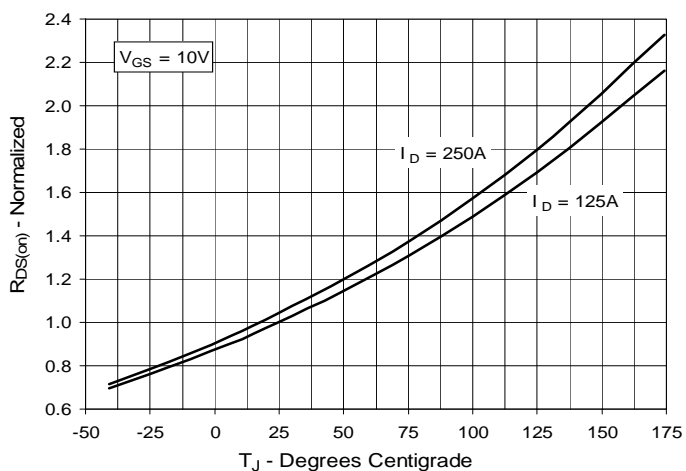
Fig. 4. R_{DS(on)} Normalized to I_D = 125A Value vs. Junction Temperature
