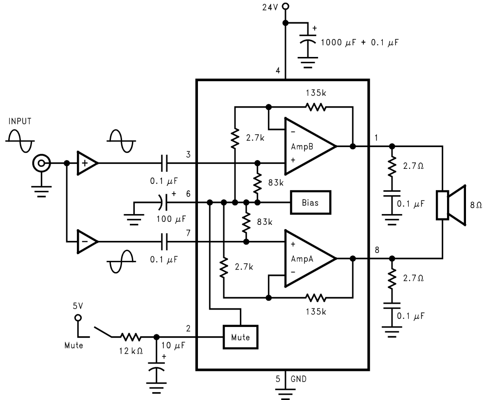
FIGURE 4. Bridge-Mode Application
