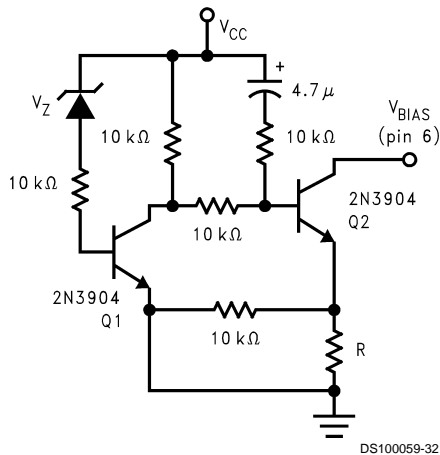
FIGURE 6. External Undervoltage Pull-Down
