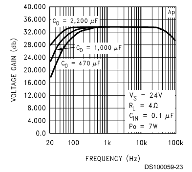
Frequency Response
