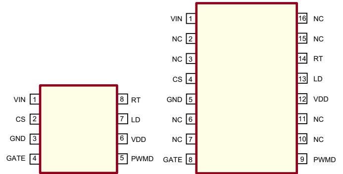
8-Lead SOIC (LG)
