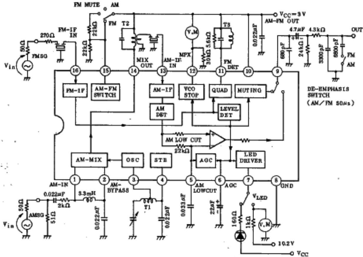
TEST CIRCUIT 1
