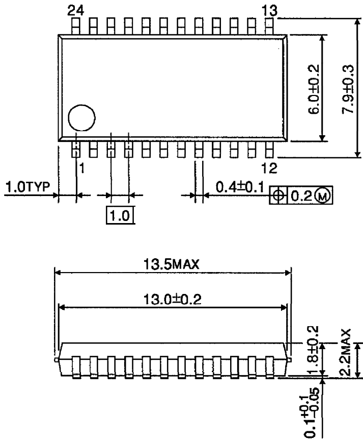
OUTLINE DRAWING SSOP24-P-300-1.00
