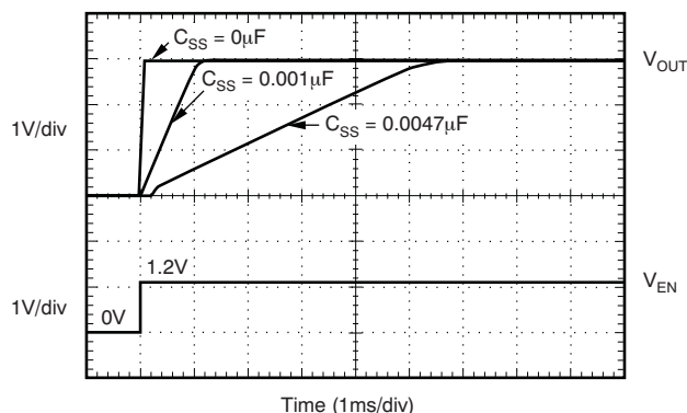
Figure 2. Turn-On Response
