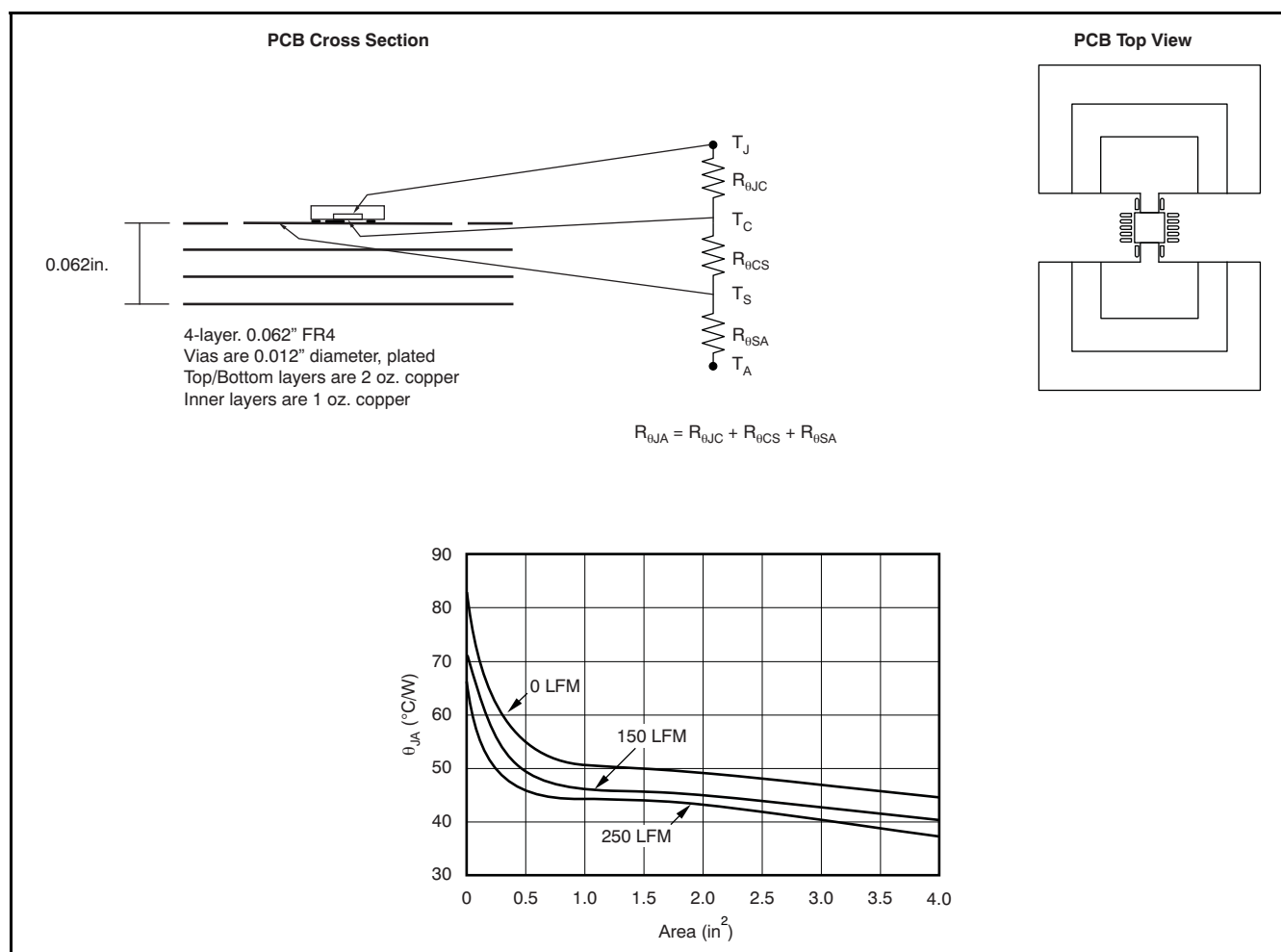
Figure 32. PCB Layout and Corresponding R_{\theta JA} Data, Top Layer Only
