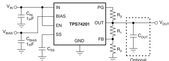
Figure 1. Typical Application Circuit for the TPS74201 (Adjustable)
