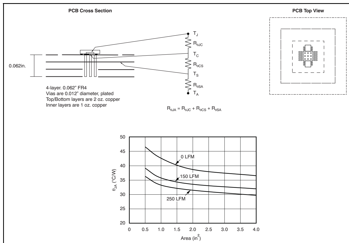
Figure 31. PCB Layout and Corresponding R_{\theta JA} Data, Vias Under Thermal Pad
