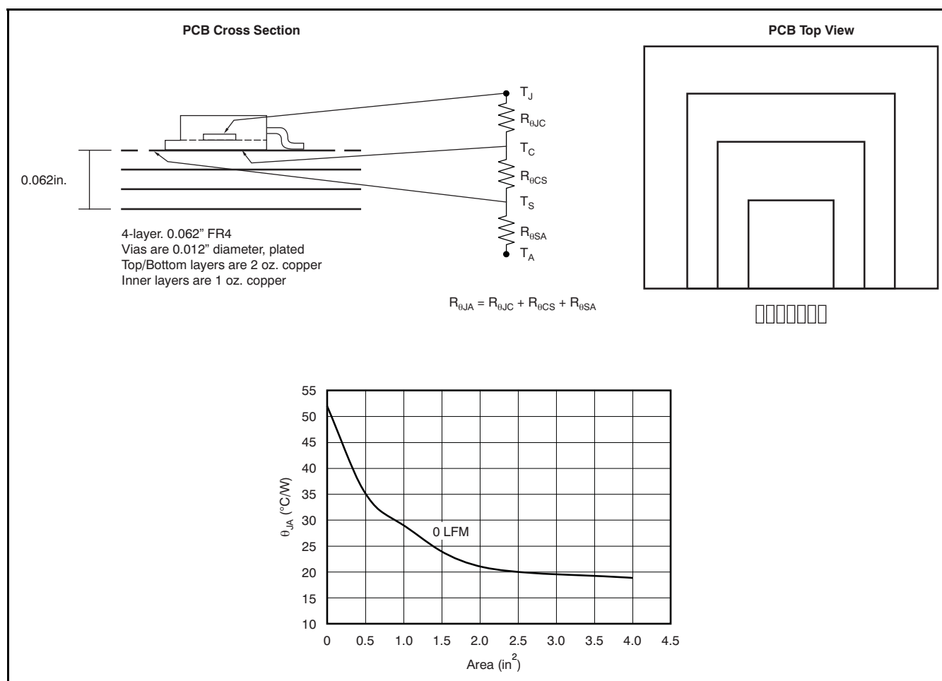
Figure 34. PCB Layout and Corresponding R_{\theta JA} , Top Layer Thermal Plane
