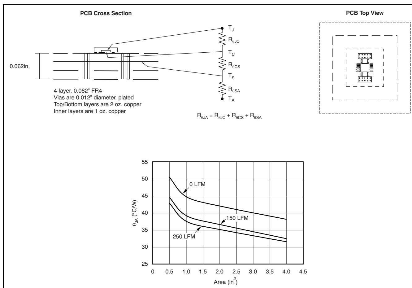
Figure 30. PCB Layout and Corresponding R_{\theta JA} Data, No Vias Under Thermal Pad
