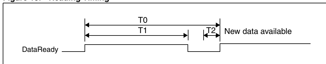
Figure 15. Reading Timing
