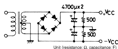
Specified transformer power supply (Equivalent to MG-200)
