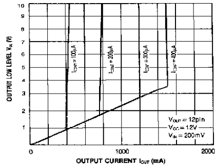
Fig. 16 OUTPUT LOW LEVEL vs. OUTPUT CURRENT
