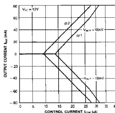
Fig. 15 OUTPUT CURRENT vs. CONTROL CURRENT
