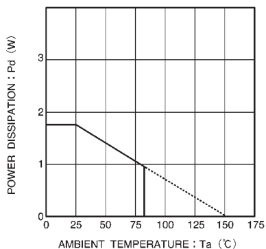
Fig.5 Thermal derating curve
