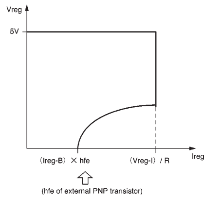
Fig.4 Regulator current limiting characteristics
