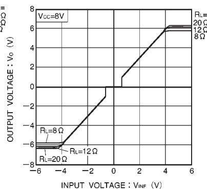
Fig.7 Loading driver I / O characteristics (channels 3 and 6)
