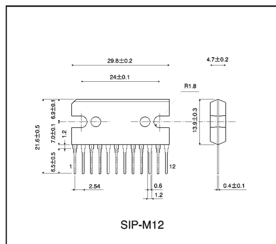
●External dimensions (Units: mm)
