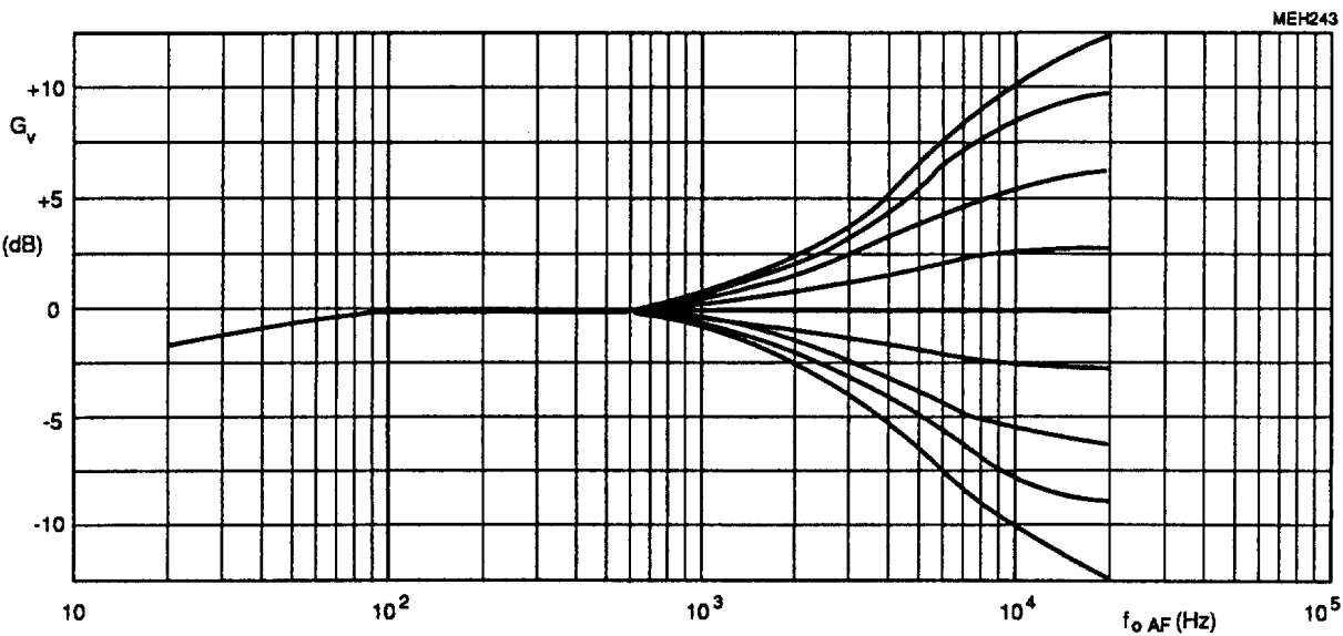
Fig.7 Treble control.
