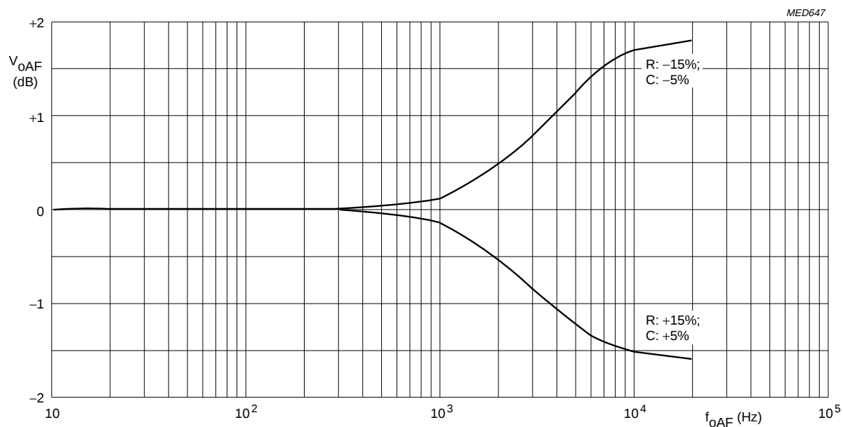
Fig.4 Tolerance scheme of AF frequency response; de-emphasis with C_{D1}, C_{D2} = 10 \text{ nF } (\pm 5\%) , R_{internal} = 5 \text{ k}\Omega (\pm 15\%) .
