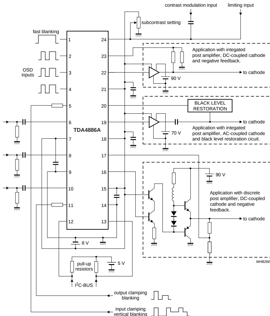
Fig.15 Basic applications for different kinds of post amplifiers with DC or AC coupling.
