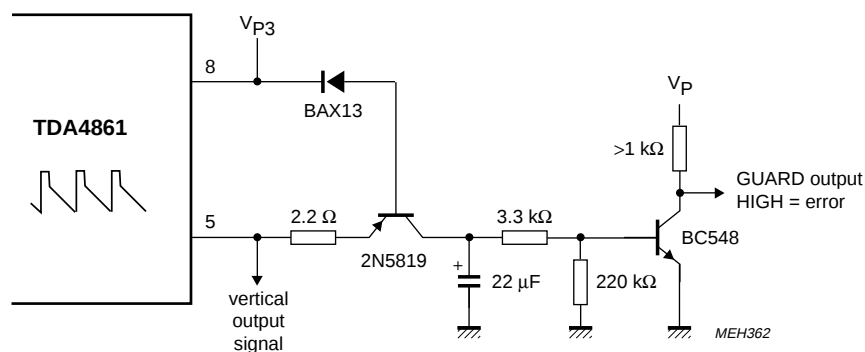
Fig.4 GUARD circuit application on vertical output.
