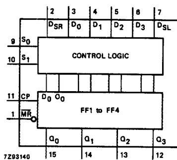
Fig.4 Functional diagram.
