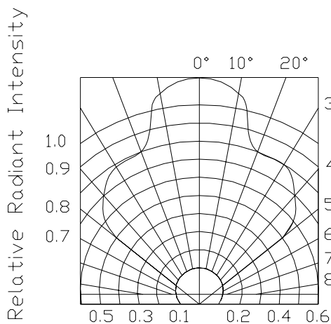
VIEW ANGLE EP204K-150XX
