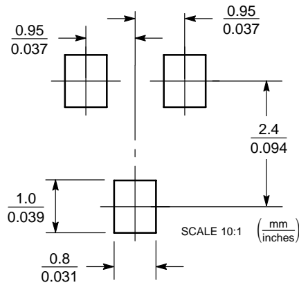
Figure 35. SC-59
