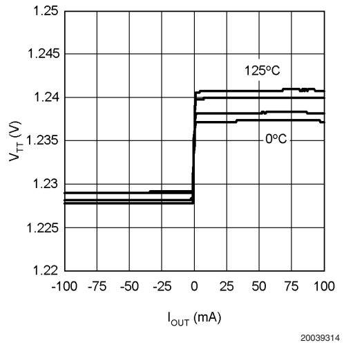
V TT vs I OUT (0, 25, 85, and 125°C)
