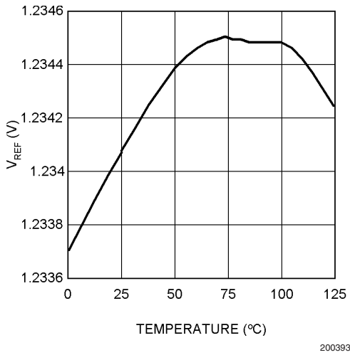
V REF vs Temperature (No Load)
