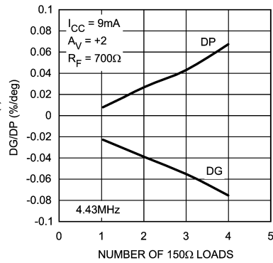
DG/DP for Various R L I CC = 9mA
