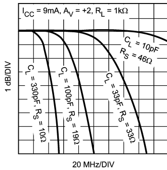
Frequency Response for Various C_L I_{CC} = 9\text{mA}
