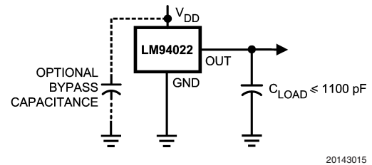
FIGURE 2. LM94022 No Decoupling Required for Capacitive Loads Less than 1100 pF.
