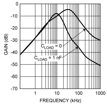
Supply-Noise Gain vs. Frequency
