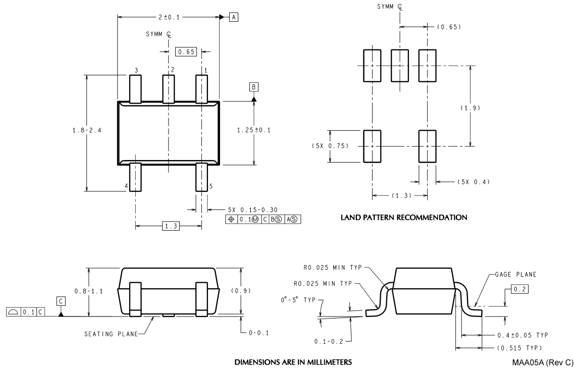
5-Lead SC70 Molded Package Order Number LM94022BIMG, LM94022BIMGX NS Package Number MAA05A
