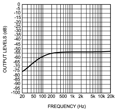
Channel Separation R_L = 16\Omega , P_O = 5\text{mW} Single Ended Output, A_V = -1
