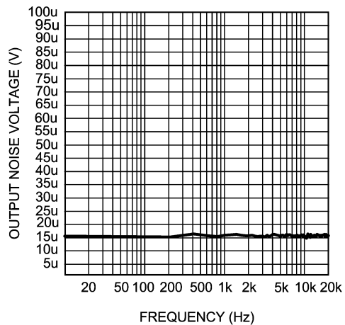
Noise Floor V_{DD} = 1.5V , BTL Output 8\Omega , 80kHz Bandwidth
