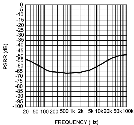
Power Supply Rejection Ratio V_{DD} = 1.5\text{V} , V_{RIPPLE} = 200\text{mV}_{PP} R_L = 8\Omega , BTL Input Terminated into 10\Omega
