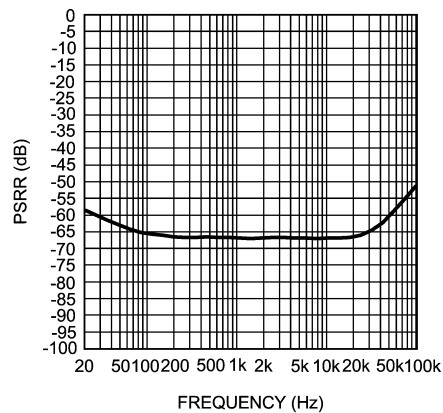
Power Supply Rejection Ratio V_{DD} = 1.2\text{V} , V_{RIPPLE} = 200\text{mV}_{PP} R_L = 16\Omega , Single Ended Output Input Terminated into 10\Omega
