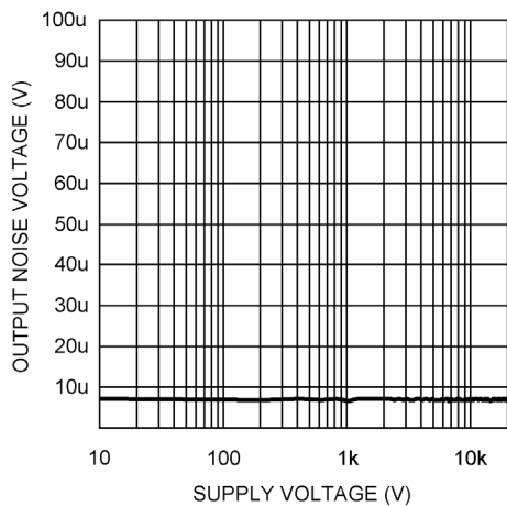
Noise Floor V_{DD} = 1.5V , Single Ended Output 16\Omega , 80kHz Bandwidth
