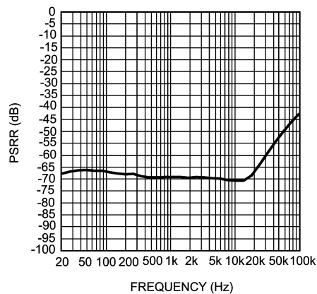
Power Supply Rejection Ratio V_{DD} = 1.5\text{V} , V_{RIPPLE} = 200\text{mV}_{PP} R_L = 16\Omega , Single Ended Output Input Terminated into 10\Omega
