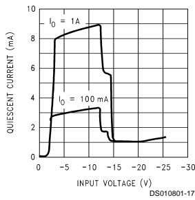
LM2990-12 Quiescent Current
