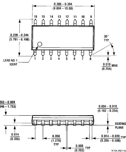
16-Lead Molded Small Outline Package (M) Order Number DS26C32ATM NS Package Number M16A
