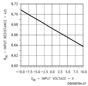
Input Resistance vs Input Voltage
