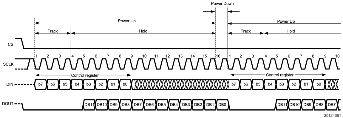
ADC124S021 Operational Timing Diagram
