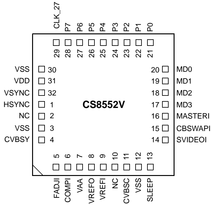
Figure-1 32-pin PLCC
