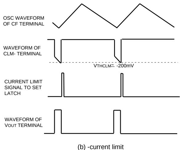
Fig.11 Operating waveforms of current limiting circuit
