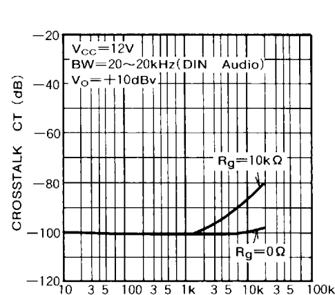
CROSSTALK VS. FREQUENCY CHARACTERISTICS
