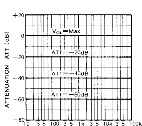
ATTENUATION VS. FREQUENCY CHARACTERISTICS
