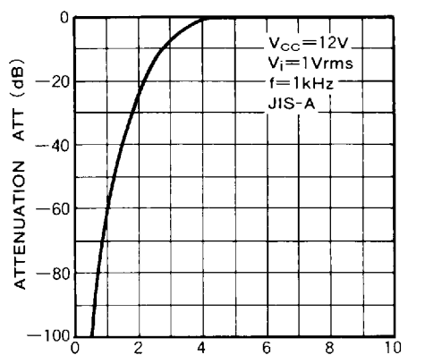
ATTENUATION VS. VOLUME CONTROL
