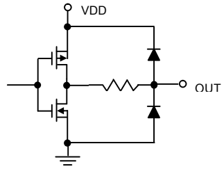
SDO terminal
