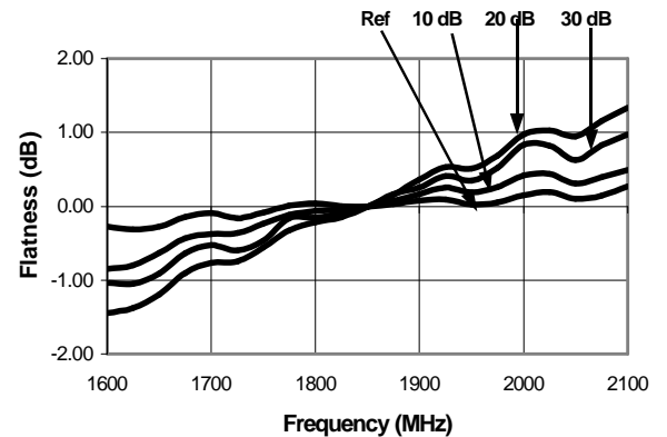
Attenuation Flatness (dB) @ +25°C
