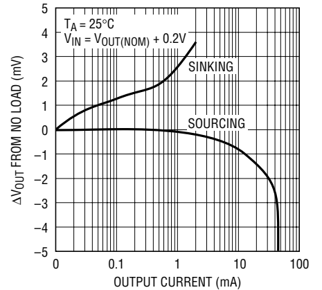
LTC1258 Series Load Regulation
