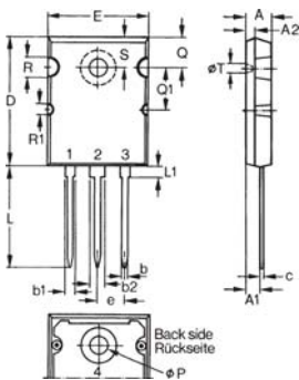
TO-264 Outline
