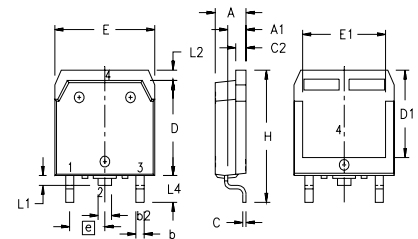
TO-268 (IXTT) Outline
