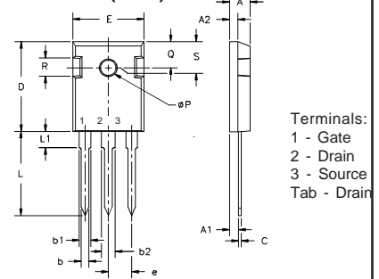
TO-247 AD (IXFH) Outline
