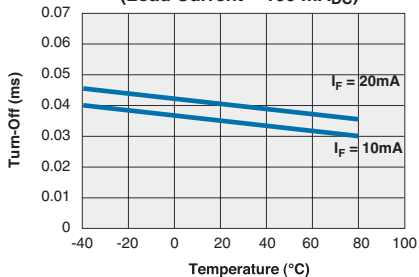
CPC1926Y Typical Turn-Off vs. Temperature (Load Current = 100 mA DC )
