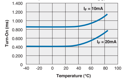
CPC1926Y Typical Turn-On vs. Temperature (Load Current = 100 mA DC )
