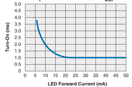
CPC1926Y Typical Turn-On vs. LED Forward Current (Load Current = 100 mA DC )
