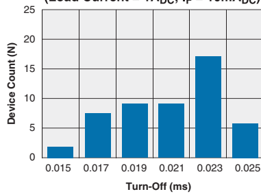
CPC1926Y Typical Turn-Off Time (N=50 Ambient Temperature = 25°C) (Load Current = 1A DC ; I_F = 10\text{mA}_{DC} )
