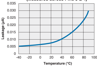
CPC1926Y Typical Leakage vs. Temperature at Maximum Rated Voltage (Measured across Pins 3 & 4)
