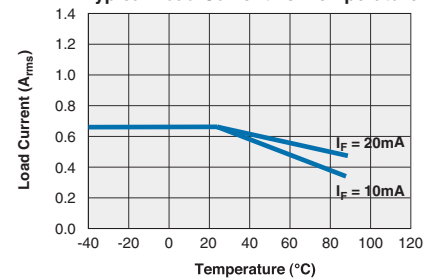
CPC1926Y Typical Load Current vs. Temperature
