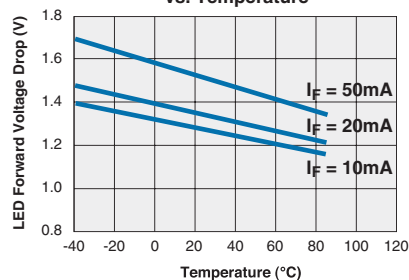
CPC1926Y Typical LED Forward Voltage Drop vs. Temperature
