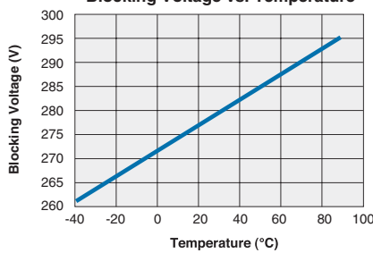
CPC1926Y Blocking Voltage vs. Temperature
