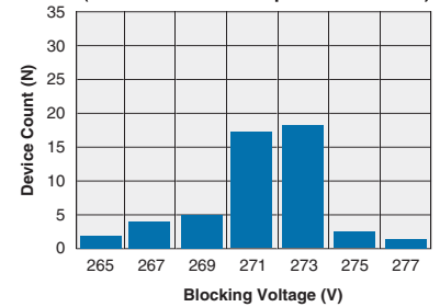
CPC1926Y Typical Blocking Voltage Distribution (N=50 Ambient Temperature = 25°C)
